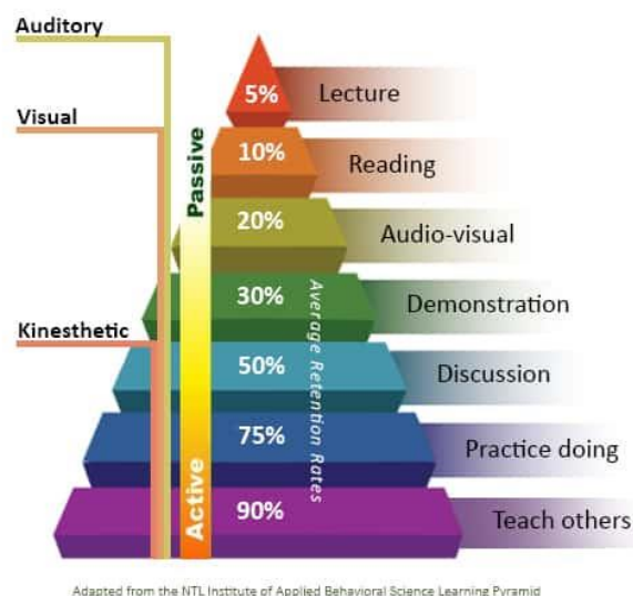
Fig 1. Learning Pyramid
