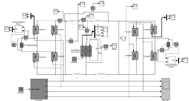
Fig. 2. Simulink diagram of dual converter fed DC motor drive
