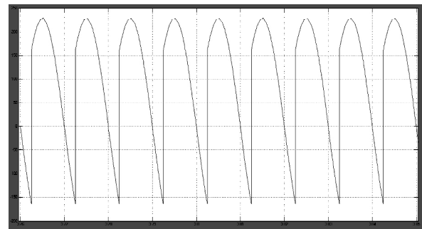
Fig. 3. Output voltage across Rectifier
