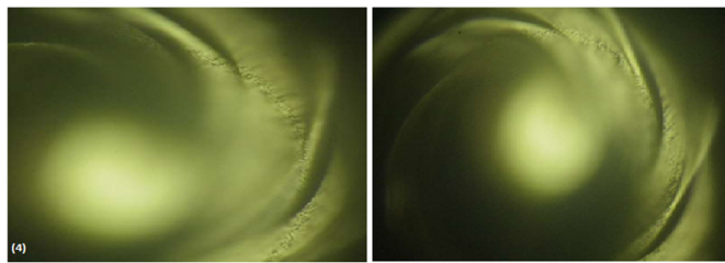
Fig 4. Crack formation caused by the extremely high pressure from gas expansion during firing
