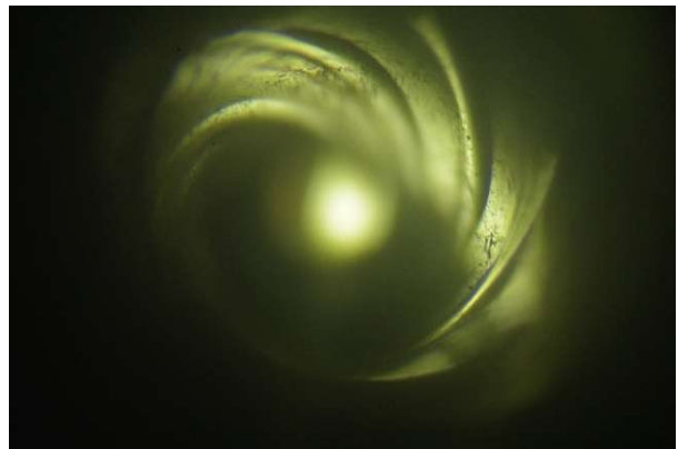
Fig 3. Narrow crack formation starting to propagate at the gun Barrel's Throat region
