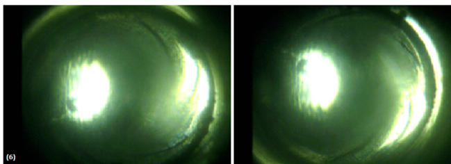
Fig 6. Superficial scraped surface due to metal-to-metal rubbing which causes corrosion and sliding wear
