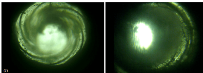
Fig 7. Presence of heavy soot particles around the gun barrel caused by continuous use of the firearm
