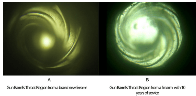
Fig 2. Side by side comparison of gun barrels' throat region with contrasting service usage
