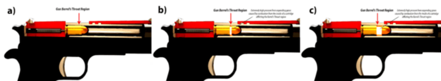
Fig 1. Illustration of a launching procedure of a projectile causing wear at the Gun Barrel's Throat Region: (a) before the exit of high-pressure gas (b) first impact of high-pressure gas to the barrel's throat region (c) maximum impact of high-pressure gas to the barrel's throat region
