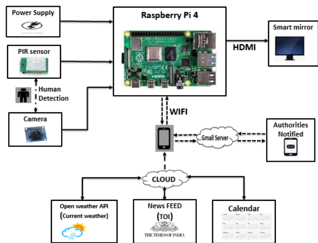
Fig 4. Proposed architecture
