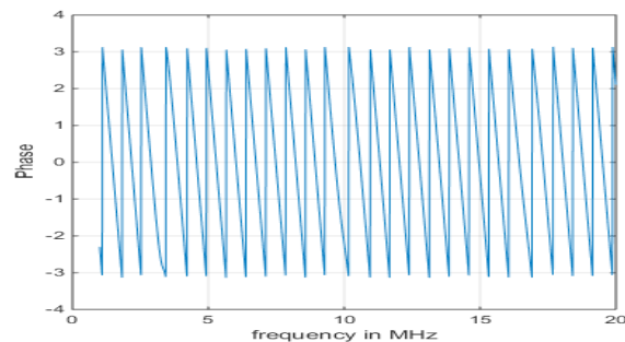
Figure 7. PLC channel model for phase (N=4).
