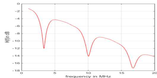
Figure 6. PLC channel model for gain (N=4).
