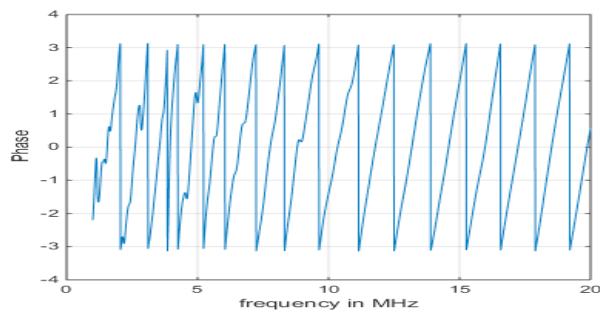
Figure 9. PLC channel model for phase (N=15).
