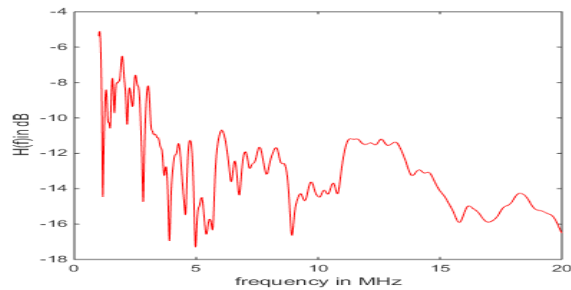
Figure 8. PLC channel model for gain (N=15).
