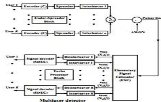
Figure 10. IDMA Transmitter and receiver structure with k simultaneous users for power line.
