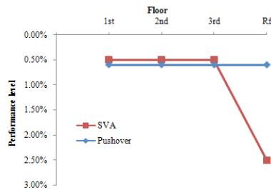
Figure 5. Comparison between SVA and pushover analysis model e.
