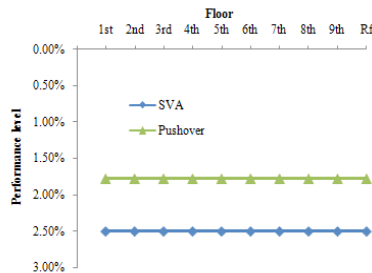
Figure 3. Comparison between SVA and pushover analysis model c.
