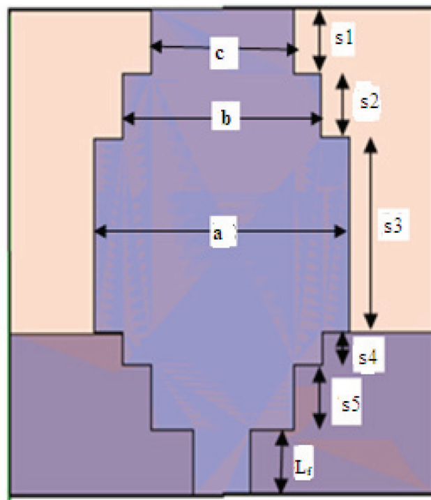
Figure 9. Geometry of proposed antenna.s
