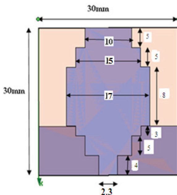
Figure 14. Detailed dimensions of Proposed Antenna.
