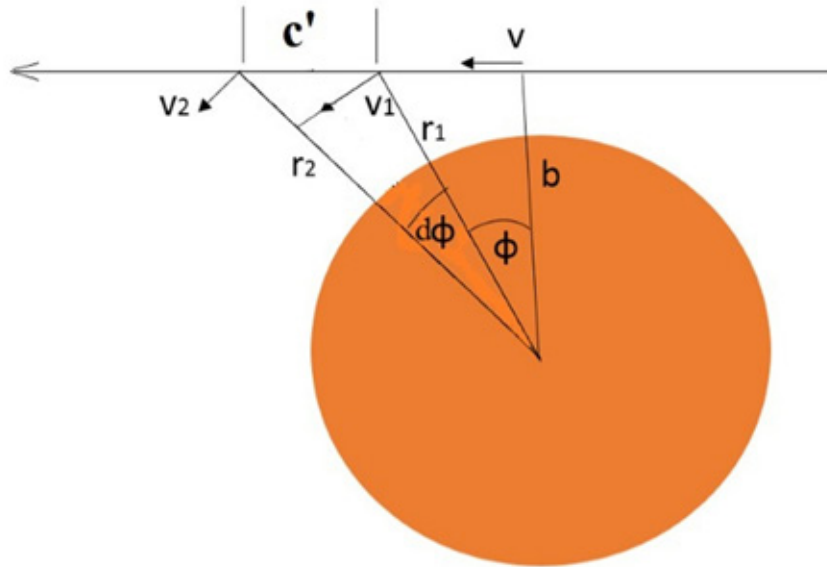
Figure 8. Orbital velocities in the path of light at two points apart by a distance equal to c' .
