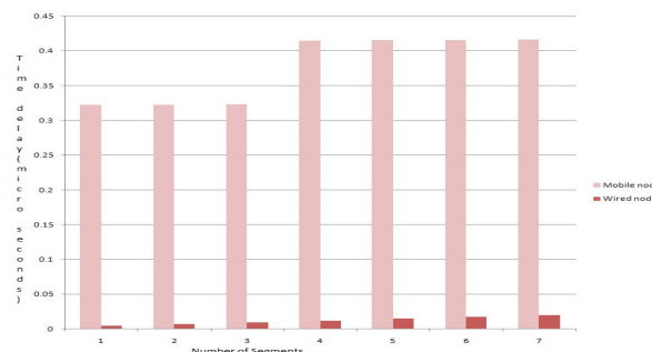
Figure 9. Performance of the wired and the mobile nodes.
