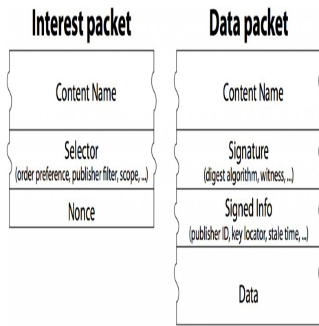
Figure 2. Interest and Data packet formats.
