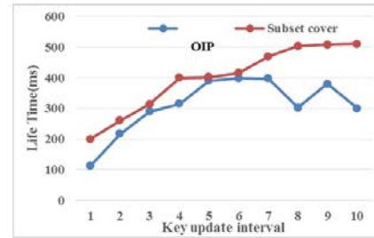
Figure 7. Average lifetime vs. key update interval.
