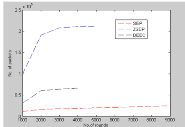
Figure 7. No. of packets transmitted in FAIR, LEACH, SEP, ZSEP, DEEC for a = 1 , m = 0.2 .
