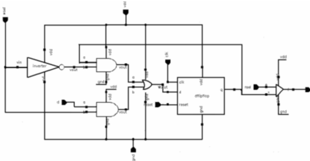
Figure 7. 1-bit accumulator.
