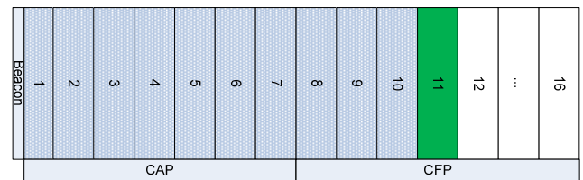
Figure 4. Simple scenario with single data in superframe generating in CFP region.
