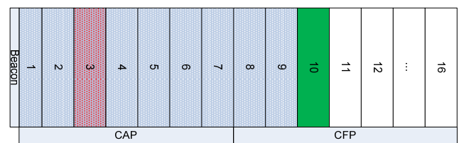
Figure 3. Simple scenario with single data in superframe generating in CAP region.
