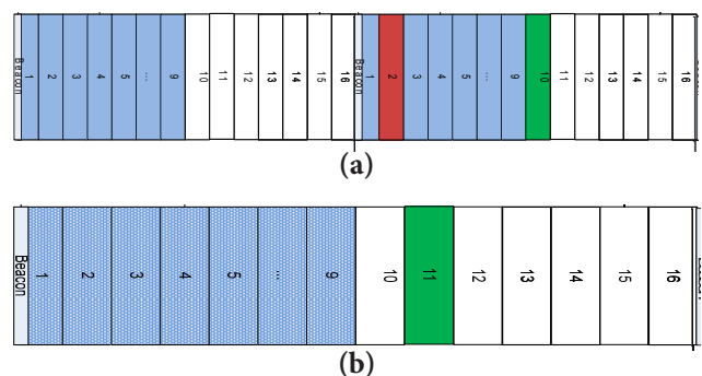
Figure 6. Comparison total delay of a data in two different BO and SO selection. (a) Considering two successive superframe with BO=SO=0. (b) Consider one superframe with Bo=SO=1.
