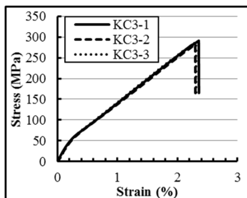
Figure 8. Stress-strain behaviour of KC3 hybrid composite plate.
