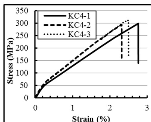
Figure 9. Stress-strain behaviour of KC4 hybrid composite plate.
