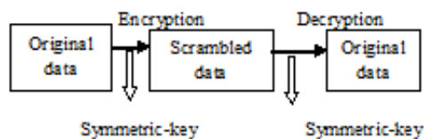
Figure 2. Symmetric-Key Cryptography.
