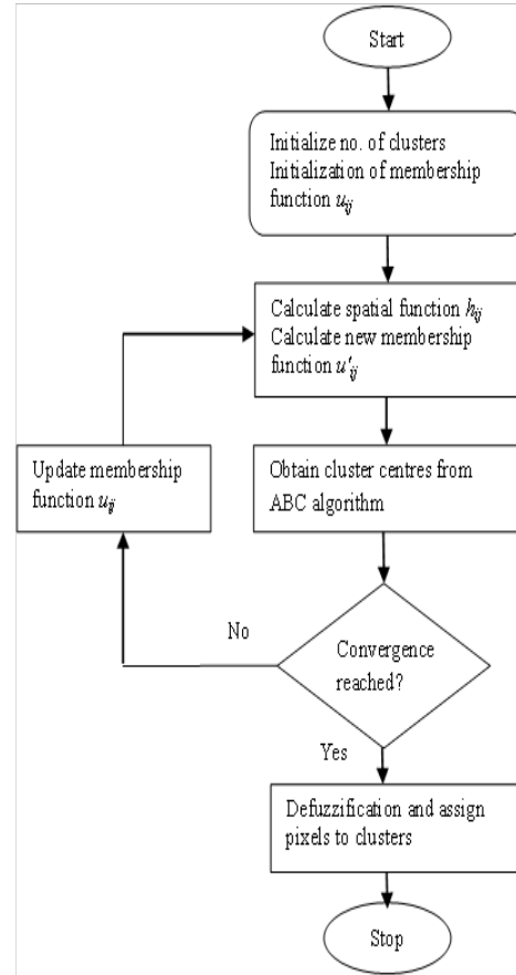
Figure 3. ABCSFCM algorithm.
