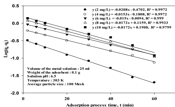
Figure 7. First order Kinetic model for adsorption of Cd on to WTAC as adsorbent.
