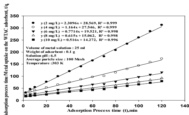
Figure 8. Second order Kinetic model for adsorption of Cd on to WTAC as adsorbent.
