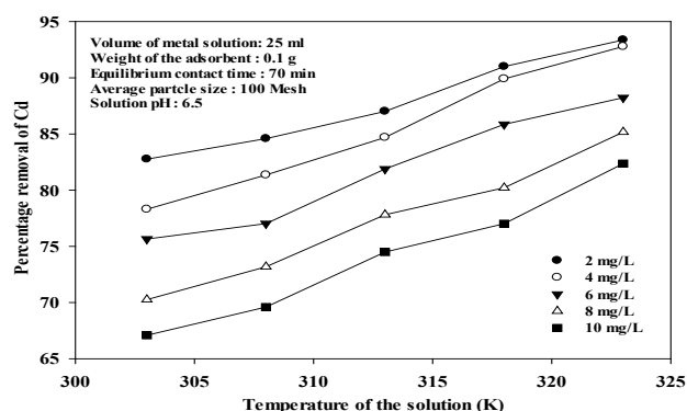
Figure 5. Effect of temperature on percentage removal of Cd onto WTAC adsorbent.
