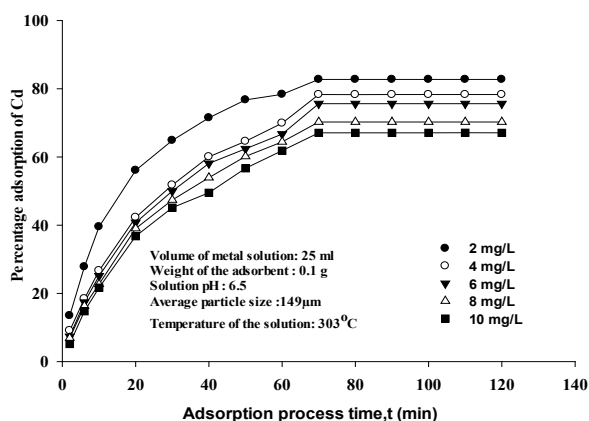
Figure 1. Effect of adsorption process time on % adsorption of Cd using WTAC as an adsorbent.
