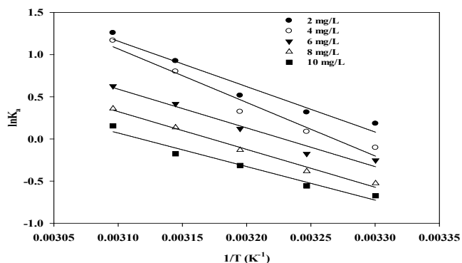
Figure 6. Plot for estimation of thermodynamic energy properties using Van't- Hoffrelation
