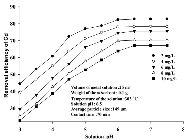
Figure 2. Effect of solution pH on the removal efficiency of Cd using WTAC as an adsorbent.
