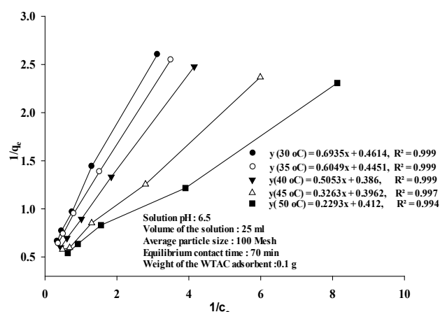
Figure 4. Langmuir isotherms at four different temperatures for the removal of Cd.
