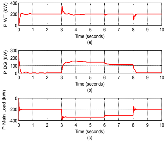
Figure 3. Real power at (a) wind turbine terminal, (b) diesel genset terminal and (c) main load terminal.
