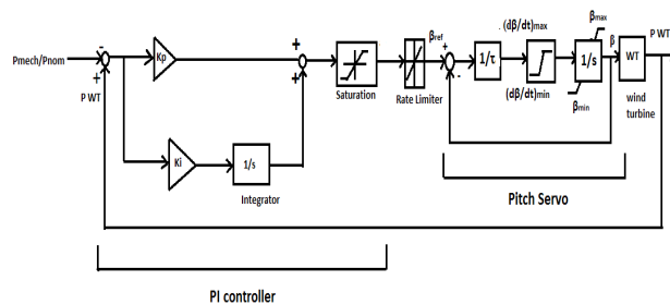
Figure 13. Block diagram of pitch angle control incorporating PI controller with pitch servo.
