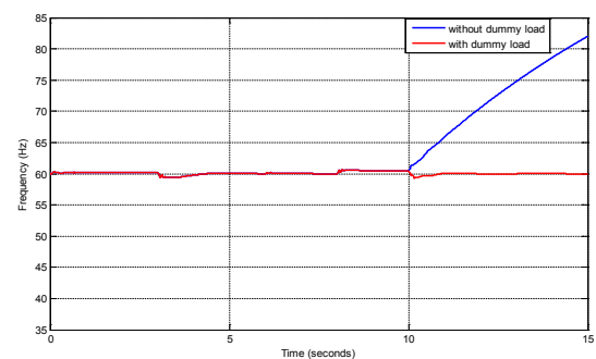
Figure 8. Frequency of synchronous generator of diesel genset without and with dummy load.
