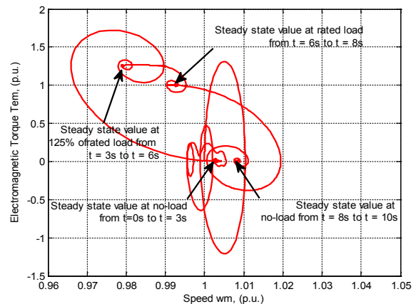
Figure 5. Speed ( w_m ) vs. electromagnetic torque ( T_{em} ) characteristics of heavy load.
