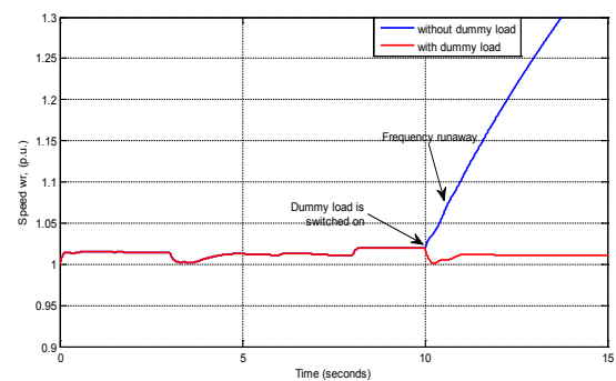
Figure 7. Speed of SEIG ( w_r ) driven by wind turbine without and with dummy load.
