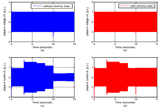
Figure 9. Instantaneous voltage of phase A ( v_A ) at main load terminal, (a) Without dummy load, (b) With dummy load and instantaneous current of phase A ( i_A ) at main load terminal, (c) without dummy load and (d) with dummy load.
