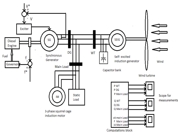
Figure 1. Modified schematic diagram of IW-D Hybrid System feeding static load and heavy load.
