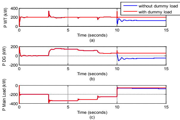
Figure 10. Real power at (a) wind turbine terminal, (b) diesel genset terminal and (c) main load terminal without and with dummy load.
