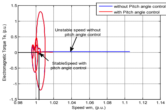
Figure 18. Speed ( w_m ) vs. electromagnetic torque ( T_{em} ) characteristics of heavy load without and with pitch angle control.
