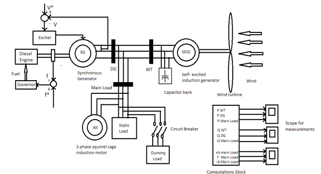
Figure 6. Modified schematic diagram of IW-D Hybrid System feeding static load, heavy load along with dummy load.
