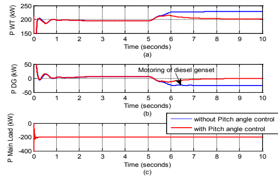
Figure 15. Real power at (a) Wind turbine terminal, (b) Diesel genset terminal and (c) Main load terminal without and with pitch angle control.
