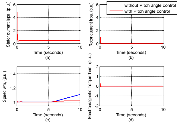
Figure 17. (a) Stator current of phase 'a' ( i_{spa} ), (b) Rotor current of phase 'a' ( i_{rpa} ), (c) Speed ( w_m ) and (d) Electromagnetic torque ( T_{em} ) of heavy load without and with pitch angle control.
