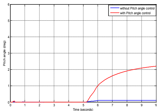
Figure 14. Pitch angle of wind turbine under varying wind speed without and with pitch angle control.
