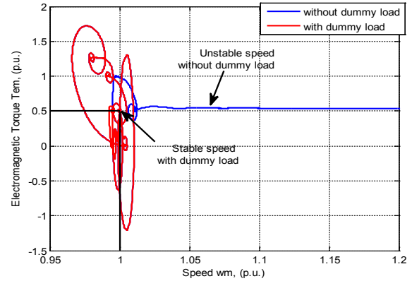
Figure 12. Speed ( w_m ) vs. electromagnetic torque ( T_{em} ) characteristics of heavy load.
