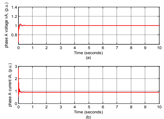
Figure 16. (a) Voltage of phase 'A' ( v_A ) at main load terminal and (b) Current of phase 'A' ( i_A ) at main load terminal without and with PI controller.
