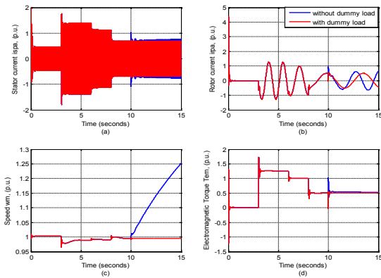
Figure 11. (a) Instantaneous stator current of phase 'a' ( i_{spa} ), (b) Instantaneous rotor current of phase 'a' ( i_{rpa} ), (c) Speed ( w_m ) and (d) Electromagnetic torque ( T_{em} ) of heavy load without and with dummy load.
