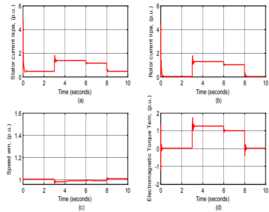
Figure 4. (a) Stator current of phase 'a' ( i_{spa} ), (b) Rotor current of phase 'a' ( i_{rpa} ), (c) Speed ( w_m ) and (d) Electromagnetic torque ( T_{em} ) of heavy load.
