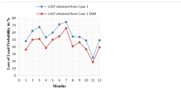
Figure 5. Comparison of LOLP obtained from both Case 1 and Case 1-DSM.
