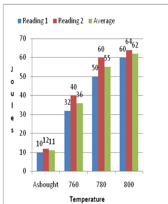
Chart 1. Impact test.
