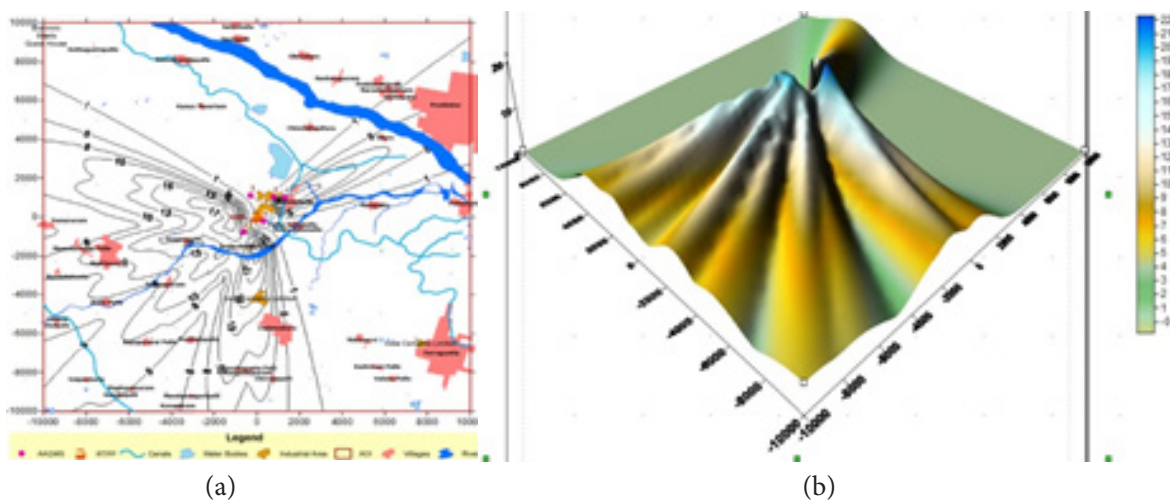
Figure 11. (a) Isopleths of \text{NO}_x in the vicinity of RTPP December 2012. (b) 3-Dimensional view of \text{NO}_x dispersion in the vicinity of RTPP December 2012.
