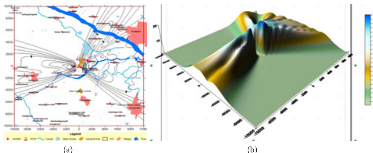
Figure 16. (a) Isopleths of NO x in the vicinity of RTPP May 2013. (b) 3-Dimensional view of NO x dispersion in the vicinity of RTPP May 2013.
