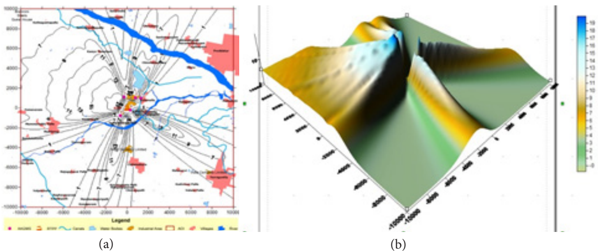
Figure 14. (a) Isopleths of \text{NO}_x in the vicinity of RTPP March 2013. (b) 3-Dimensional view of \text{NO}_x dispersion in the vicinity of RTPP March 2013.
