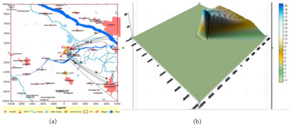
Figure 7. (a) Isopleths of \text{NO}_x in the vicinity of RTPP August 2012. (b) 3-Dimensional view of \text{NO}_x dispersion in the vicinity of RTPP August 2012.
