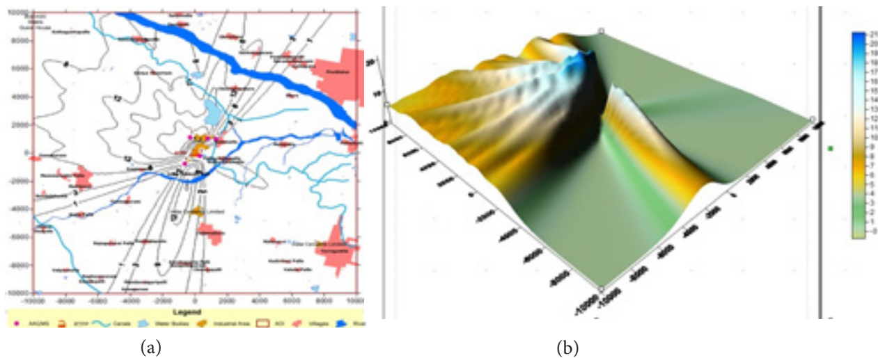
Figure 13. (a) Isopleths of \text{NO}_x in the vicinity of RTPP February 2013. (b) 3-Dimensional view of \text{NO}_x dispersion in the vicinity of RTPP February 2013.
