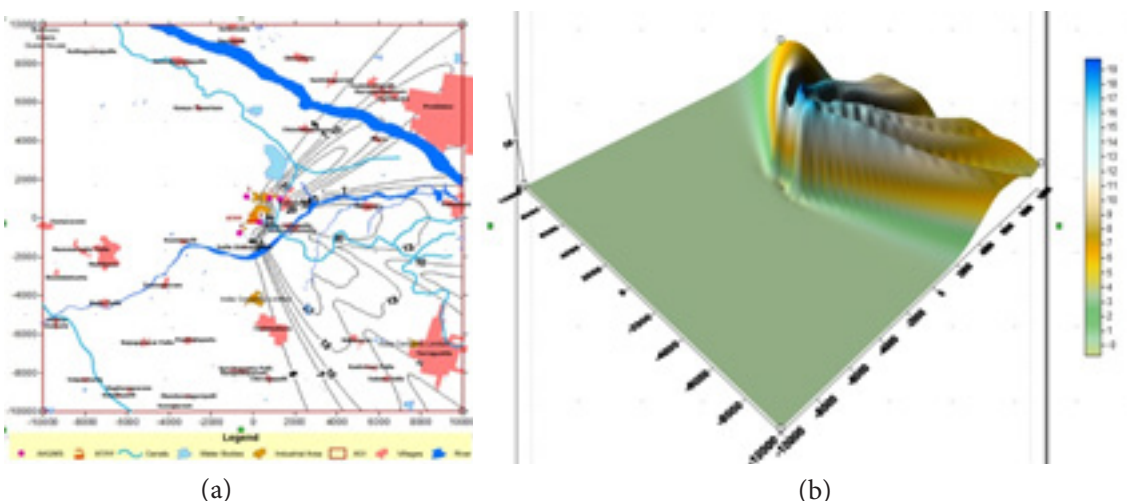
Figure 6. (a) Isopleths of \text{NO}_x in the vicinity of RTPP July 2012. (b) 3-Dimensional view of \text{NO}_x dispersion in the vicinity of RTPP July 2012.
