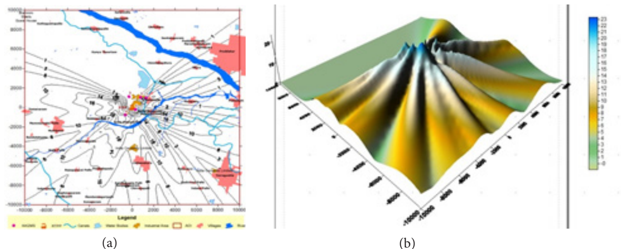
Figure 9. (a) Isopleths of \text{NO}_x in the vicinity of RTPP October 2012. (b) 3-Dimensional view of \text{NO}_x dispersion in the vicinity of RTPP October 2012.
