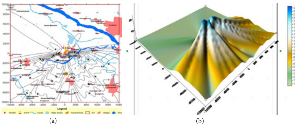
Figure 10. (a) Isopleths of \text{NO}_x in the vicinity of RTPP November 2012. (b) 3-Dimensional view of \text{NO}_x dispersion in the vicinity of RTPP November 2012.
