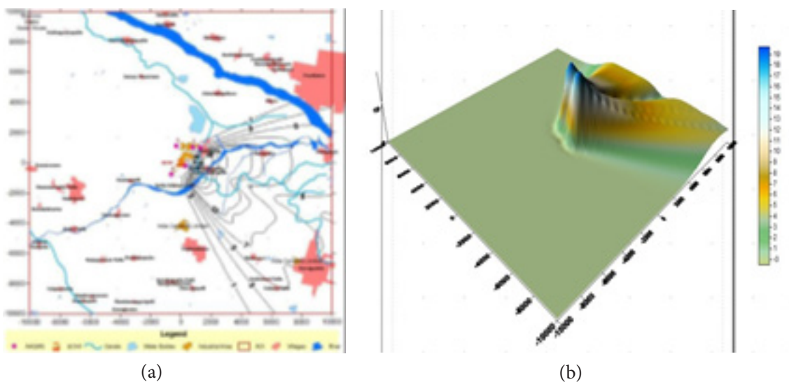
Figure 5. (a) Isopleths of \text{NO}_x in the vicinity of RTPP June 2012. (b) 3-Dimensional view of \text{NO}_x dispersion in the vicinity of RTPP June 2012.
