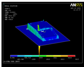
Figure 7. Simulated model for 0.018 mm clearance.
