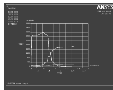
Figure 10. Energy graph for 0.028 mm clearance.
