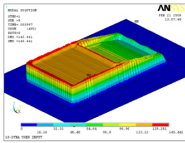
Figure 12. Simulated model for 0.028 mm clearance.
