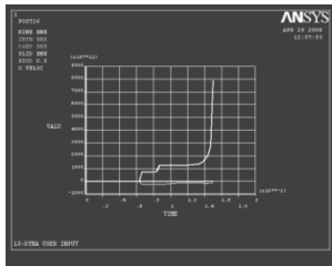
Figure 8. Energy graph for 0.018 mm clearance.
