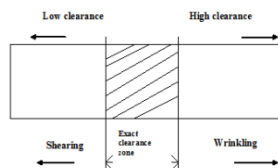
Figure 1. Effect of clearance in sheet metal forming.
