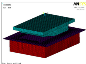
Figure 5. Meshed model.
