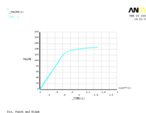
Figure 6. Load curve.
