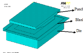
Figure 4. Assembly of punch, blank and die.
