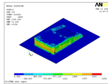
Figure 9. Simulated model for 0.028 mm clearance.
