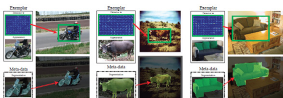
Figure 6. Segmentation Transfer.
