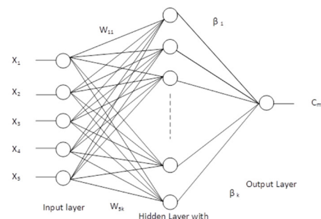
Figure 8. ELM neural network with linear nodes
