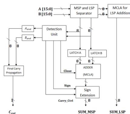
Figure 3. SPST CLA.
