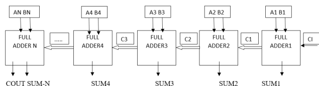
Figure 1. Parallel adder.
