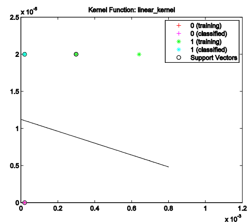
Figure 12. SVM level two classifier with linear kernel for higher order static M_{40} .
