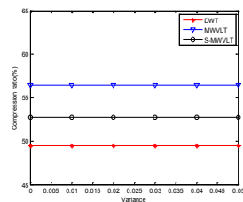
Figure 18. Compression ratio with increase in noise variance.
