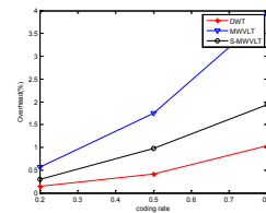
Figure 25. Overhead with variation in coding rate
