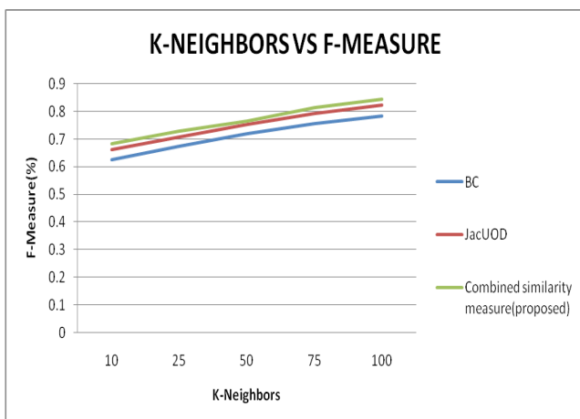
Figure 3. Comparison of F-measure against k-neighbors on web service data set.
