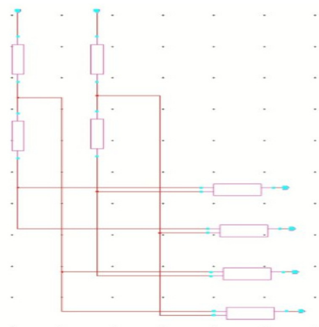
Figure 3. 2:4 NOR type decoder.
