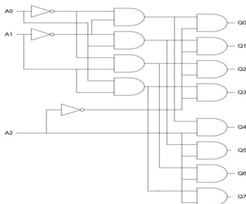
Figure 1. Traditional AND type decoders.
