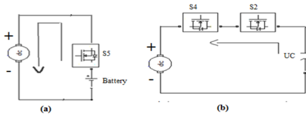
Figure 4. Quadrant I (a) Battery supplies power to load. (b) UC supplies power to load.
