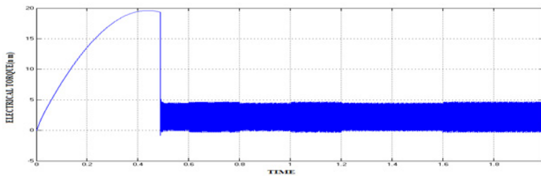
Figure 11 b. Electrical torque of a tested motor.
