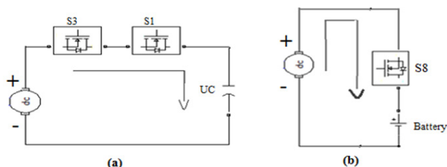
Figure 7. Quadrant II (a) Motor charges UC. (b) Motor charges Battery.
