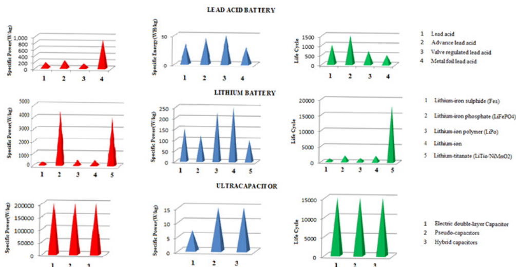
Figure 2. Battery technologies and their characteristic.
