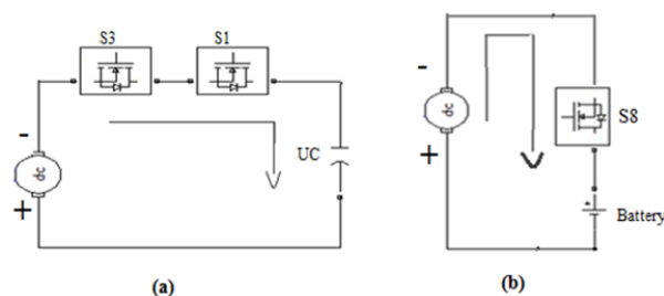
Figure 9. Quadrant IV (a) Motor charges UC. (b) Motor charges Battery.
