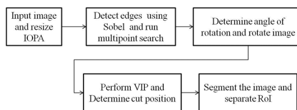
Figure 1. Block diagram of proposed algorithm
