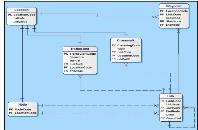
Figure 2. The entity-relationship diagram.
