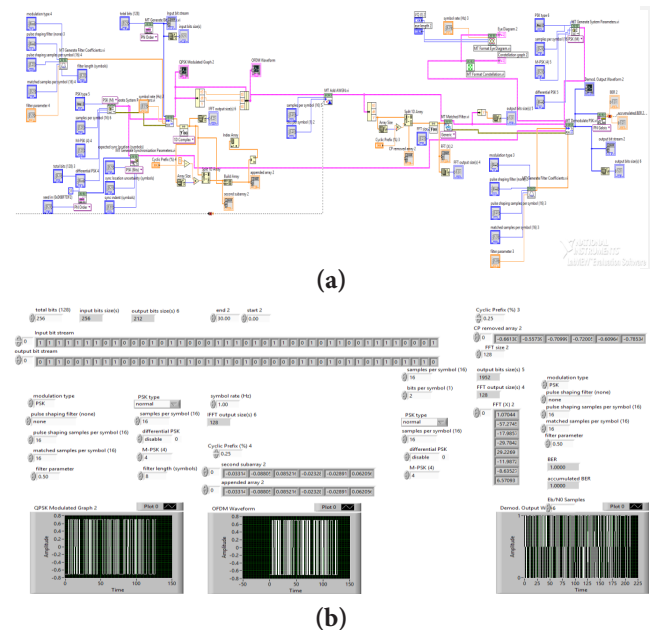
Figure 7. OFDM LabVIEW Code (a) block diagram (b) front panel.
