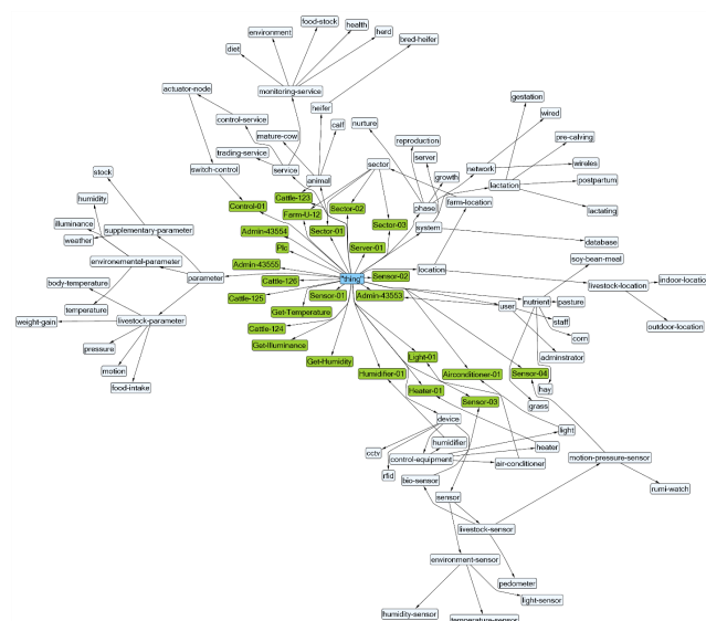
Figure 4. Basic structure of Livestock Ontology.
