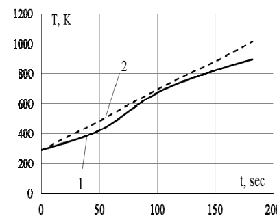
1 – ETMT with flat terminal casings having gas duct length of 29 mm, energy gain rate 0.7 W/s (Figure 15); 2 – ETMT with flat terminal casings having gas duct length of 16 mm, energy gain rate 0.4 W/s (Figure 17)
