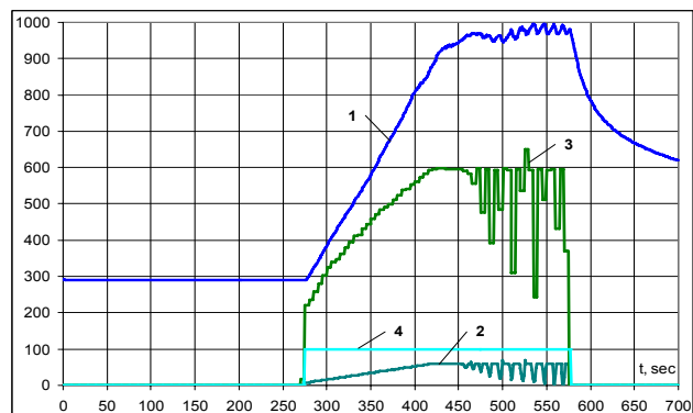
Figure 17. Time changes in the electrical parameters and temperatures for ETMT with THE: flat terminal casing; gas duct length of 16 mm; 60 W energy consumption; energy gain rate 0.4 W/s; 973 K temperature limitation
