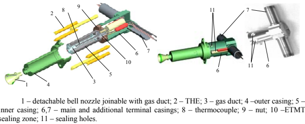
Figure 7. ETMT with cylindrical terminal casing
