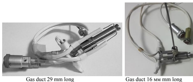
Figure 10. Experimental prototypes of ETMT with THE
