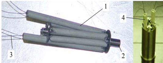
1 – two-channel ceramic tube; 2 – gas duct with nozzle; 3 – nichrome wire; 4 – THE as part of ETMT casing
