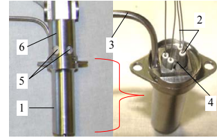
1 – ETMT; 2 – THE terminals (thermocouple terminals are not shown); 3 – ammonia feeding line; 4 – sealing cavity; 5 – sealing holes; 6 – main terminal casing.
