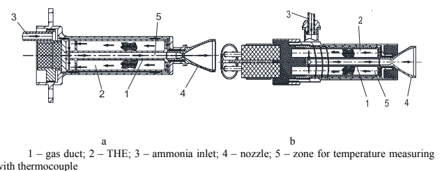
Figure 11. Scheme of ammonia flow and temperature measuring zone in ETMT with cylindrical (a) and flat (b) terminal casing
