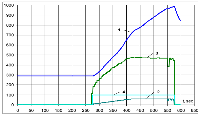
Figure 15. Time changes in the electrical parameters and temperatures for ETMT with THE: flat terminal casing; gas duct length of 29 mm; 60 W energy consumption; energy gain rate of 0.4 W/s; 987 K temperature shutdown level
