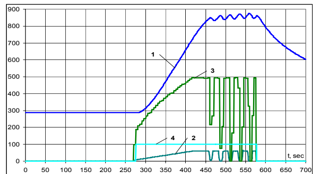
Figure 13. Time changes in the electrical parameters and pressure transducer ETMT with THE: terminal casing cylindrical; 60 W energy consumption; 0.4 W/s energy gain rate; 873 K temperature limitation
