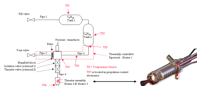
Figure 1. ETMTs manufactured by SSTL as part of CPS
