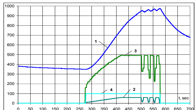
Figure 14. Time changes in the electrical parameters and temperatures for ETMT with THE: cylindrical terminal casing; 60 W energy consumption; 0.4 W/s energy gain rate; 973 K temperature limitation
