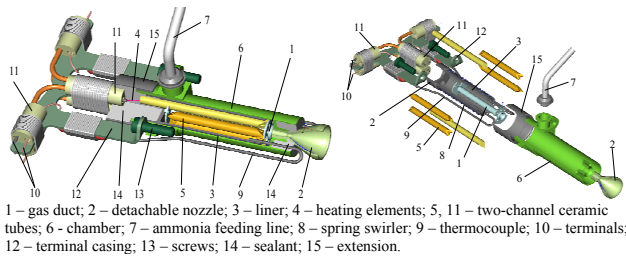
Figure 8. ETMT with flat terminal casings having gas duct length of 29 mm
