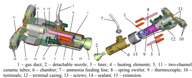
Figure 9. ETMT with flat terminal casings having gas duct length of 16 mm
