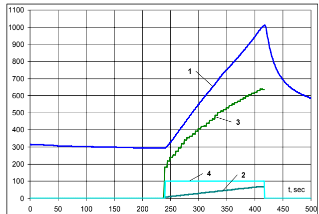
Figure 18. Time changes in the electrical parameters and temperatures for ETMT with THE: flat terminal casing; gas duct length of 16 mm; 70 W energy consumption; energy gain rate 0.4 W/s; 1013 K temperature shutdown level
