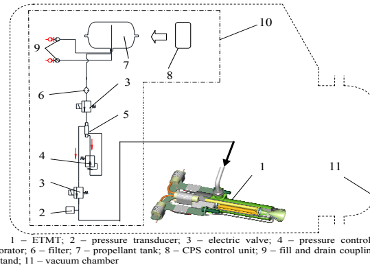
Figure 12. Scheme for testing ammonia-fueled ETMT with THE in a vacuum chamber
