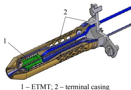
Figure 2. Xenon- fueled ETMT manufactured by SSTL
