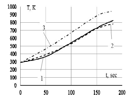
1 – ETMT with cylindrical terminal casings having gas duct length of 29 mm (Figure 12); 2 – ETMT with flat terminal casings having gas duct length of 29 mm (Figure 14); 3 – ETMT with flat terminal casings having gas duct length of 16 mm (Figure 16).
