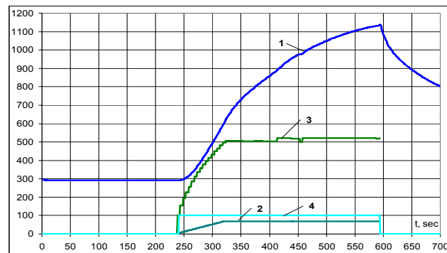
Figure 16. Time changes in the electrical parameters and temperatures for ETMT with THE: flat terminal casing; gas duct length of 29 mm; 70 W energy consumption; energy gain rate 0.7 W/s; 1133 K temperature shutdown level
