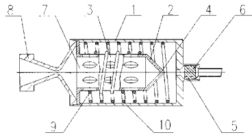
1 – fuel thermal decomposition chamber; 2 – hollow liner; 3 – perforated wall; 4 – bottom; 5 – injector; 6 – swirler; 7 – liner open end; 8 – nozzle; 9 – heater; 10 – additional heater.
