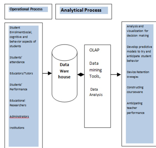
Figure 2. Architectural framework for educational data mining.
