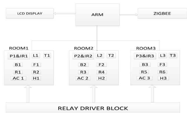
Figure 1. Proposed architecture
