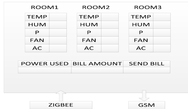
Figure 2. Monitoring section
