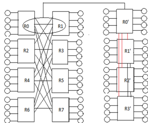
Figure 2. Flattened butterfly.
