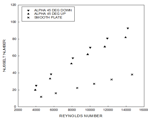
Figure 5. Variation of Reynolds number on Nusselt number with W-Discrete down and W-discrete Up ribs for angle of attack of flow of 45^\circ and relative roughness height of 0.03375.
