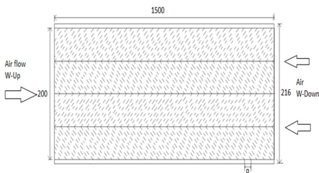
Figure 2. W-discrete ribs.
