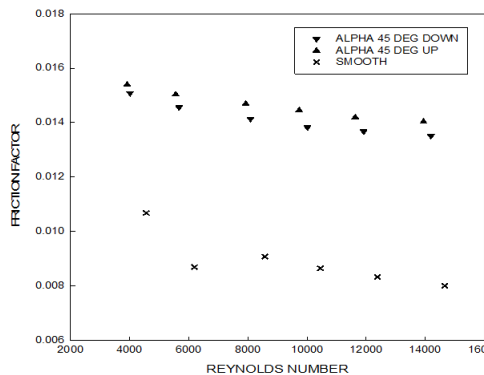
Figure 6. Variation of Reynolds number on friction factor for W-Discrete down and W-discrete Up ribs for angle of attack of flow of 45^\circ and relative roughness height of 0.03375.
