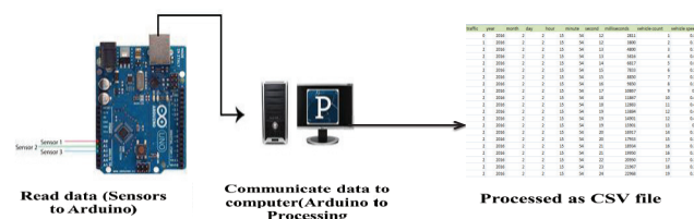
Figure 2. Converting sensor data into CSV file.
