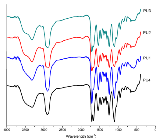
Figure 2. FTIR spectrum of the synthesized polyurethane (PU1, PU2, PU3 and PU4).
