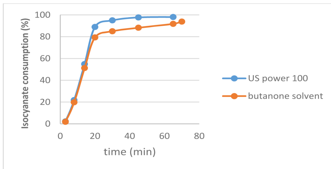
Figure 3. Effect of solvent on the consumption of NCO groups.
