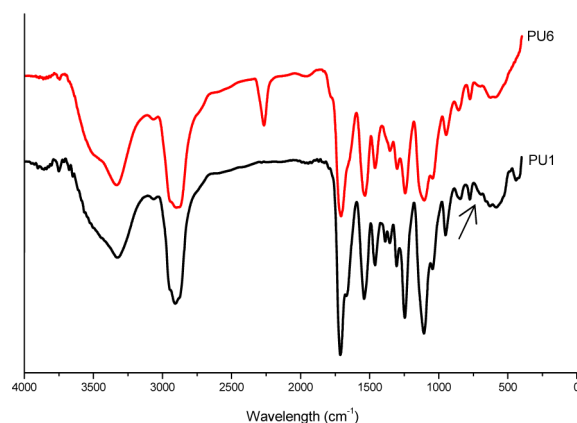
Figure 4. FTIR spectrum of the synthesized polyurethane in the presence of DMF or butanone as solvents (sonication power 100W, sonication time 30 min).
