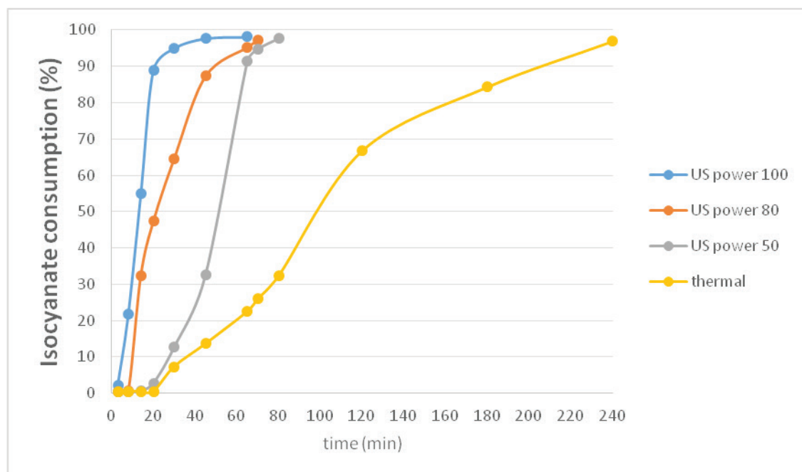
Figure 1. The effect of acoustic power and thermal polymerization on the NCO group consumption.
