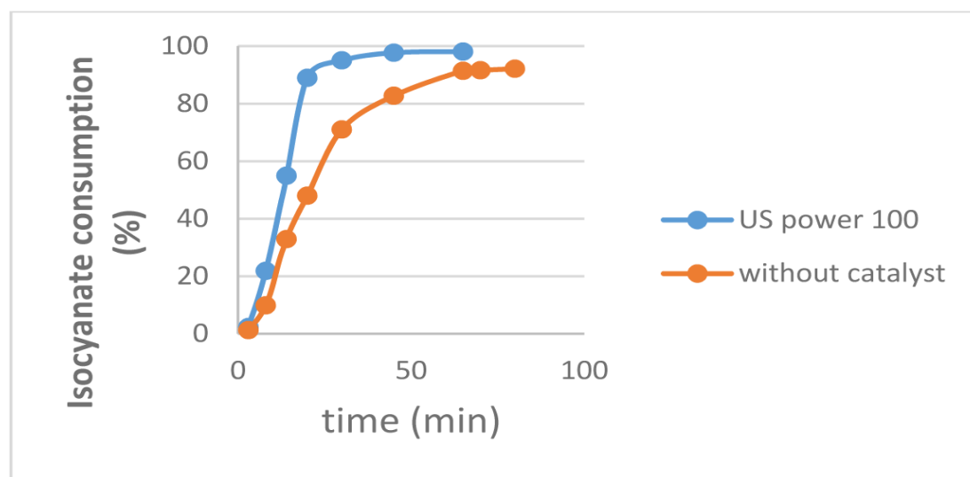
Figure 4. The effect of DBTDL catalyst on the % consumption of NCO group. (Ultrasonic power 100W).
