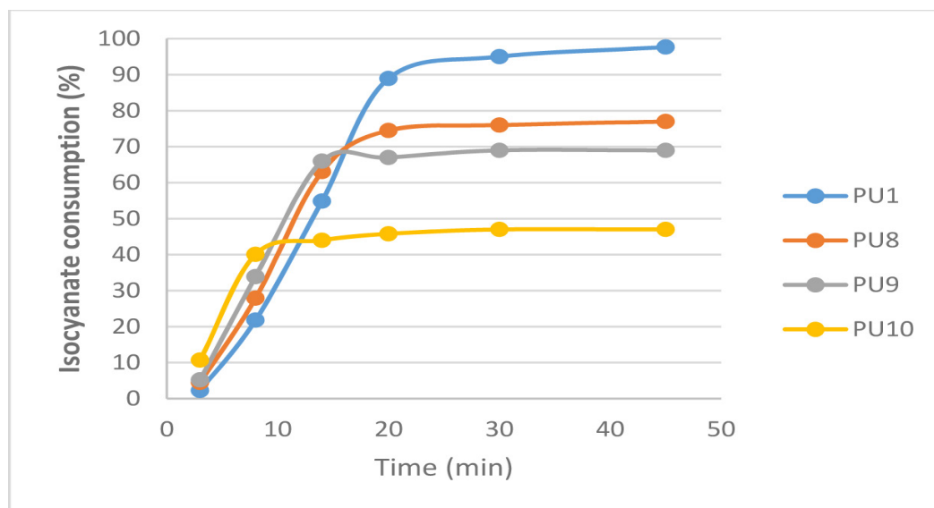
Figure 6. The effect of molar ratio of PEG, DMPA and IPDI on the % consumption of NCO group. (Ultrasonic power 100W).
