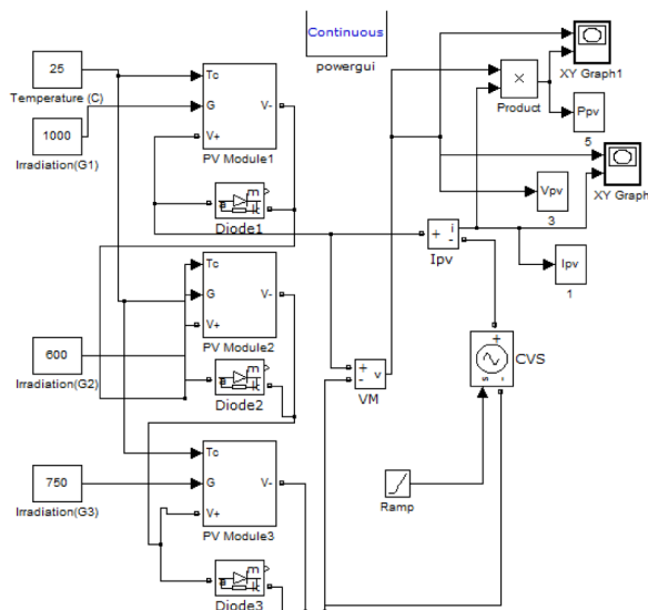
Figure 19. Simulation model of PV string.
