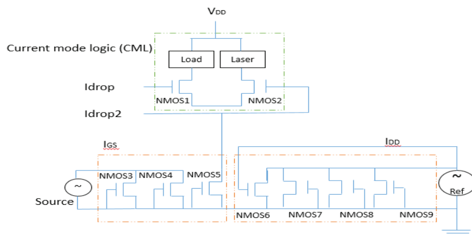
Figure 2. Semiconductor laser driver model.
