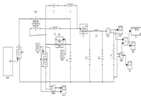
Figure 2. SEPIC converter.
