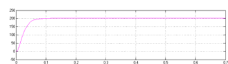
Figure 4. Output voltage of SEPIC converter.
