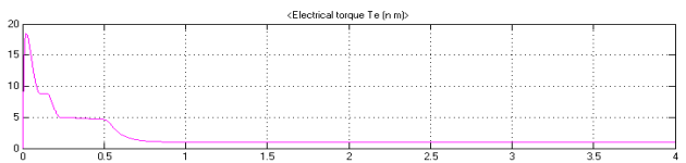
Figure 20. Torque.
