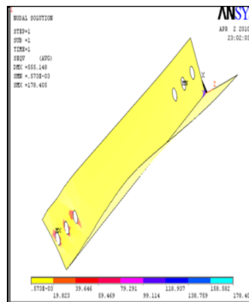
Figure 15. Stress distribution for single plain angle 50x50x2
