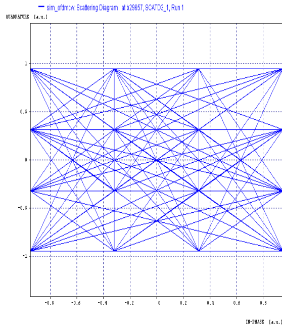
Figure 2. Scattering diagram at the transmitter.
