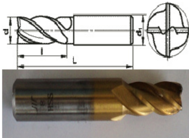
Figure 1. HSS tool ( L=69\text{mm} , l=19\text{mm} , d_1=10\text{mm} and D=8\text{mm} )
