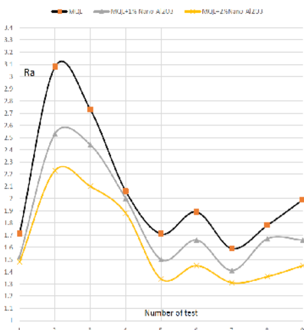
Figure 5. Diagram of surface roughness for pure MQL and MQL+nanoparticles.
