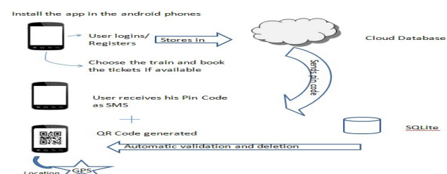
Figure 4. Dataflow diagram of ticket generation.
