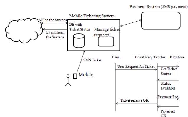
Figure 2. Use case and sequence diagram for ticket booking and checking.
