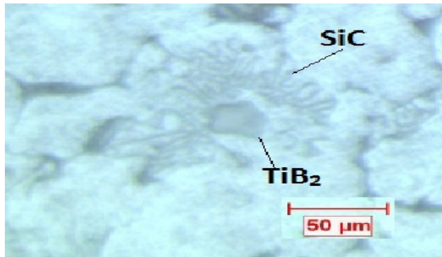
Figure 2. 10% SiC and 2.5% TiB 2 reinforcement.
