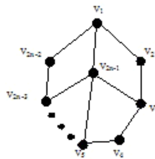
Figure 4. Jahangir Graph J_{2,n-1}
